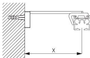
Square Smart Fix SG 11210 - SG 11215 and bracket SG 3826:
