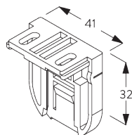
SG 10679 Bracket
